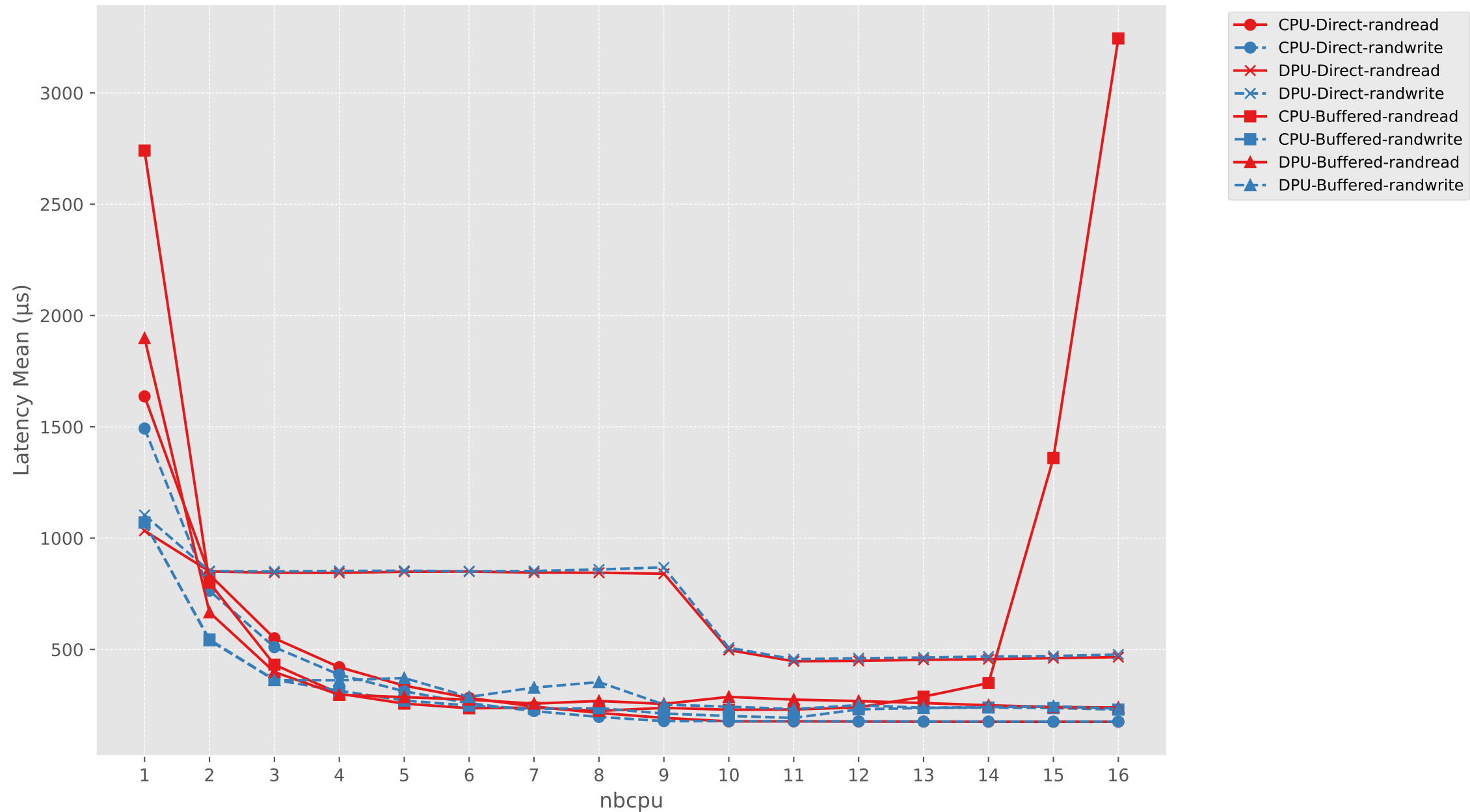
Latency Mean vs nbcpu (CPU vs DPU, Direct vs Buffered)
